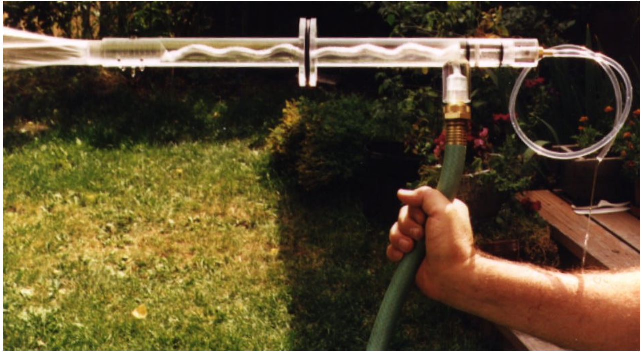
Magnetic levitation vortex trap
